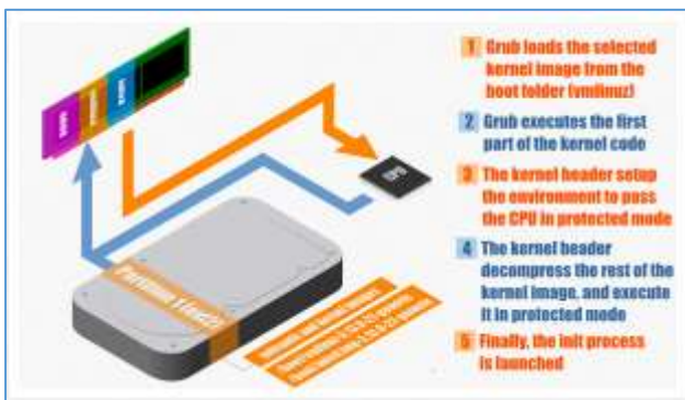
Figure 3. Major functions flow for the Linux kernel i386 boot
